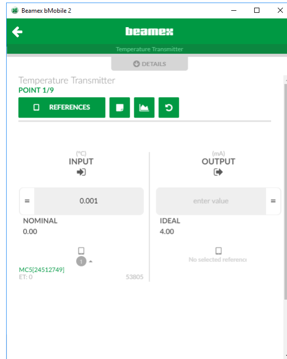
Figure 38: Calibrating a temperature transmitter
