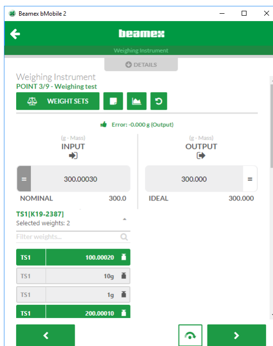
Figure 44: Weighing test of a weighing instrument
